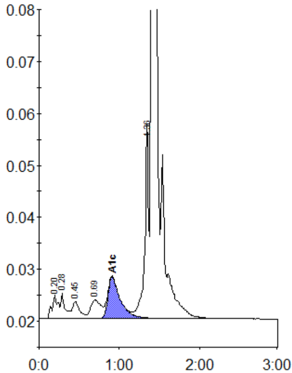
Peak table - ID: 10488028
